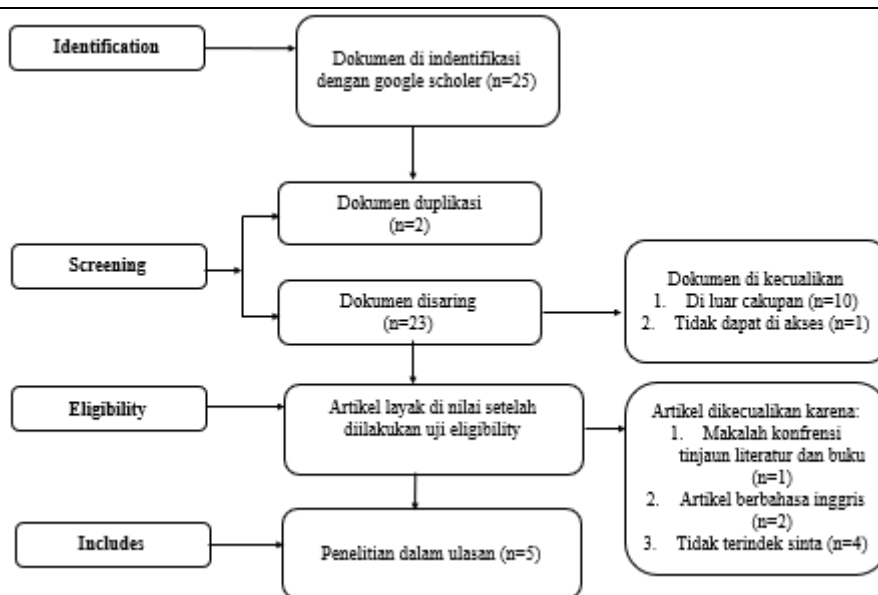
Gambar 1. Prisma Flowchart
